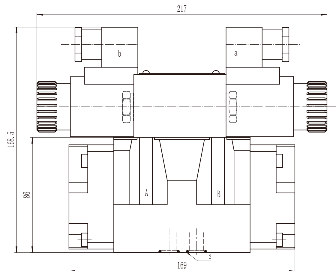
4DWHG10外型尺寸 4DWHG10 Subplate Installation Dimensions
