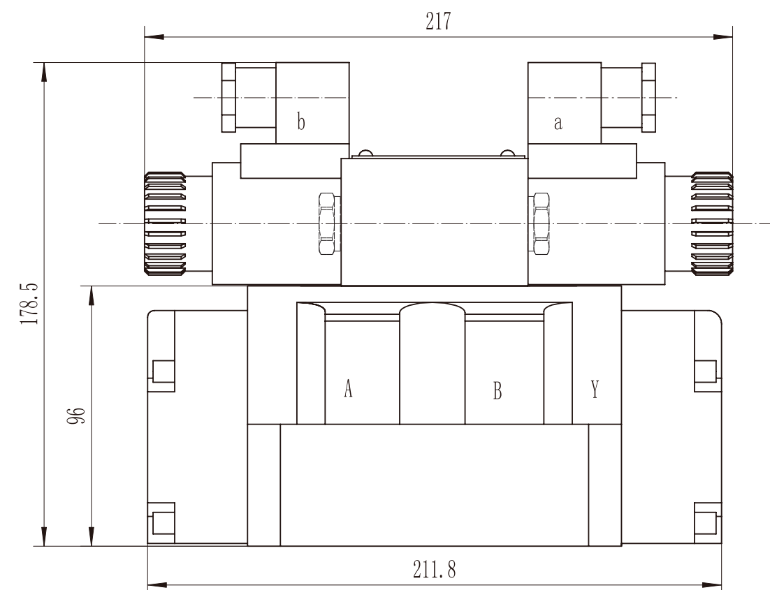
4DWHG16外型尺寸 4DWHG16 Subplate Installation Dimensions
