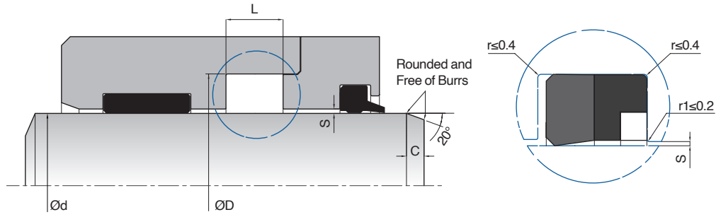
Max. Permissible Sealing Gap Value " S_{max} " (mm) for K37
