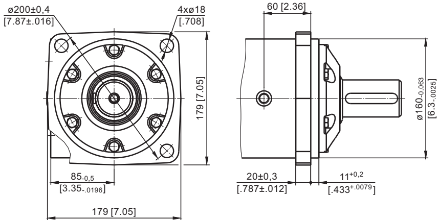
Square Mount (four holes)
