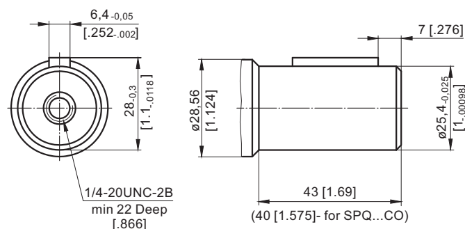
CO - \phi 1" straight, Parallel key \frac{1}{4}" \times \frac{1}{4}" \times 1" BS46 Max. Torque 34 daNm [3010 lb-in]
