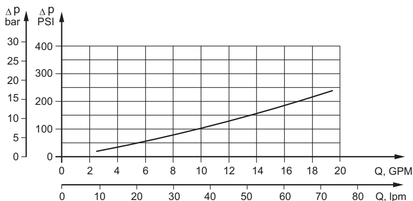
Pressure Losses
